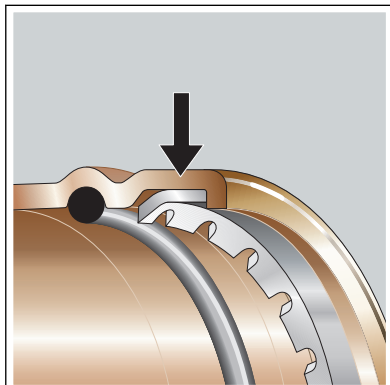
Fig. 6: Cutting ring
